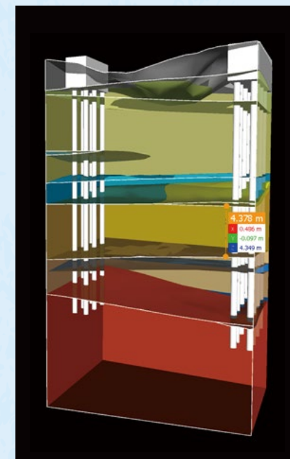
3D model of bridge foundation ground (Kyoto Prefecture)
