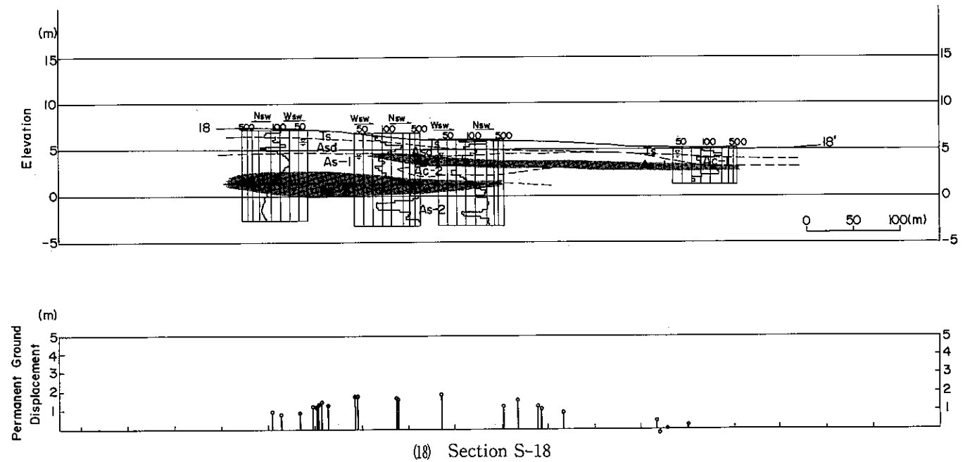
Fig. V-1 Soil layer profile in Noshiro City
