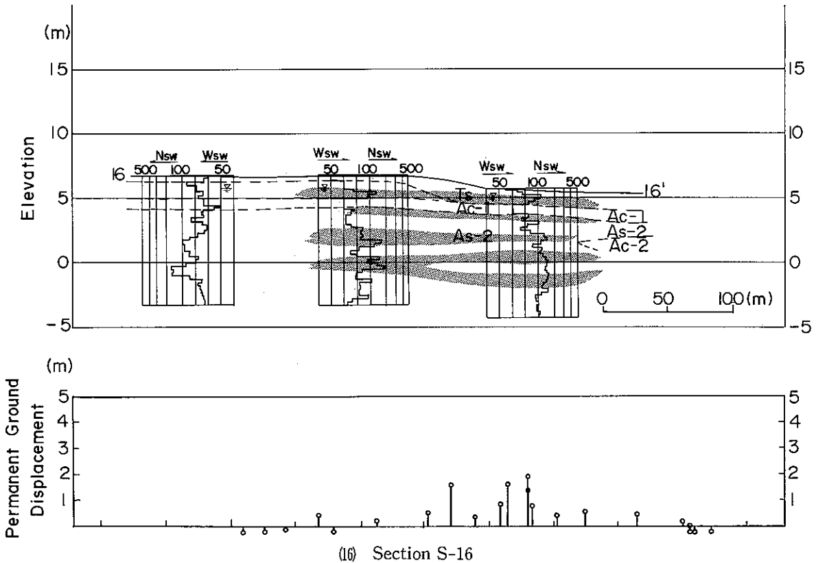
Fig. V-1 Soil layer profile in Noshiro City
