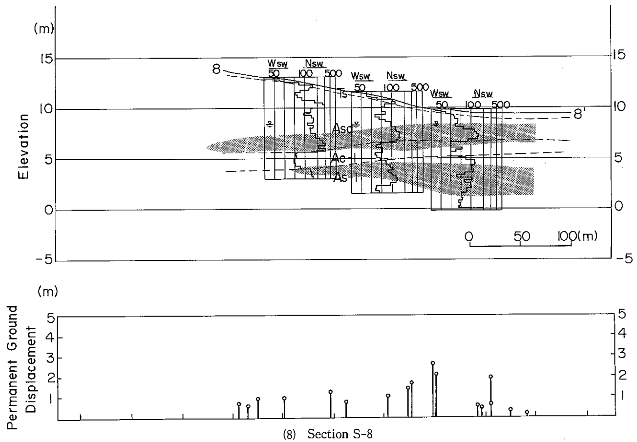
Fig. V-1 Soil layer profile in Noshiro City
