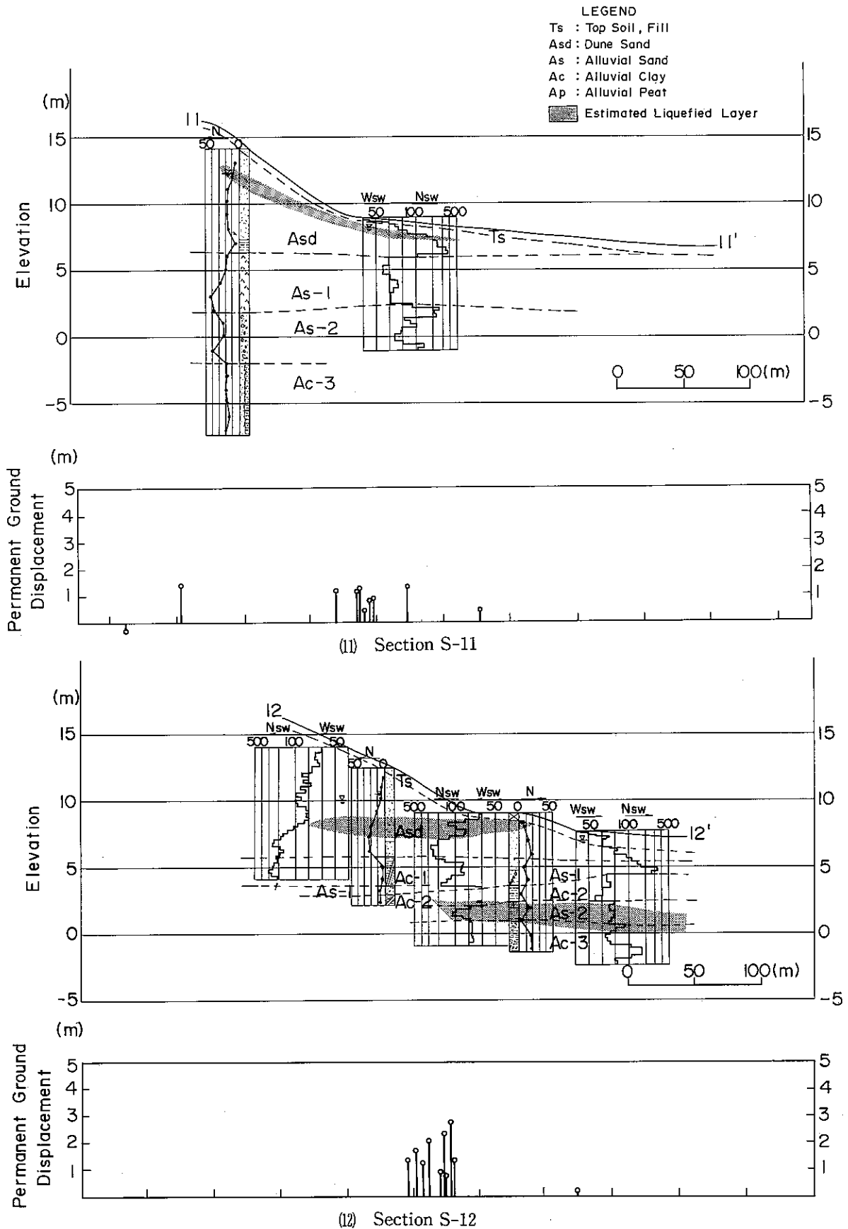
Fig. V-1 Soil layer profile in Noshiro City
