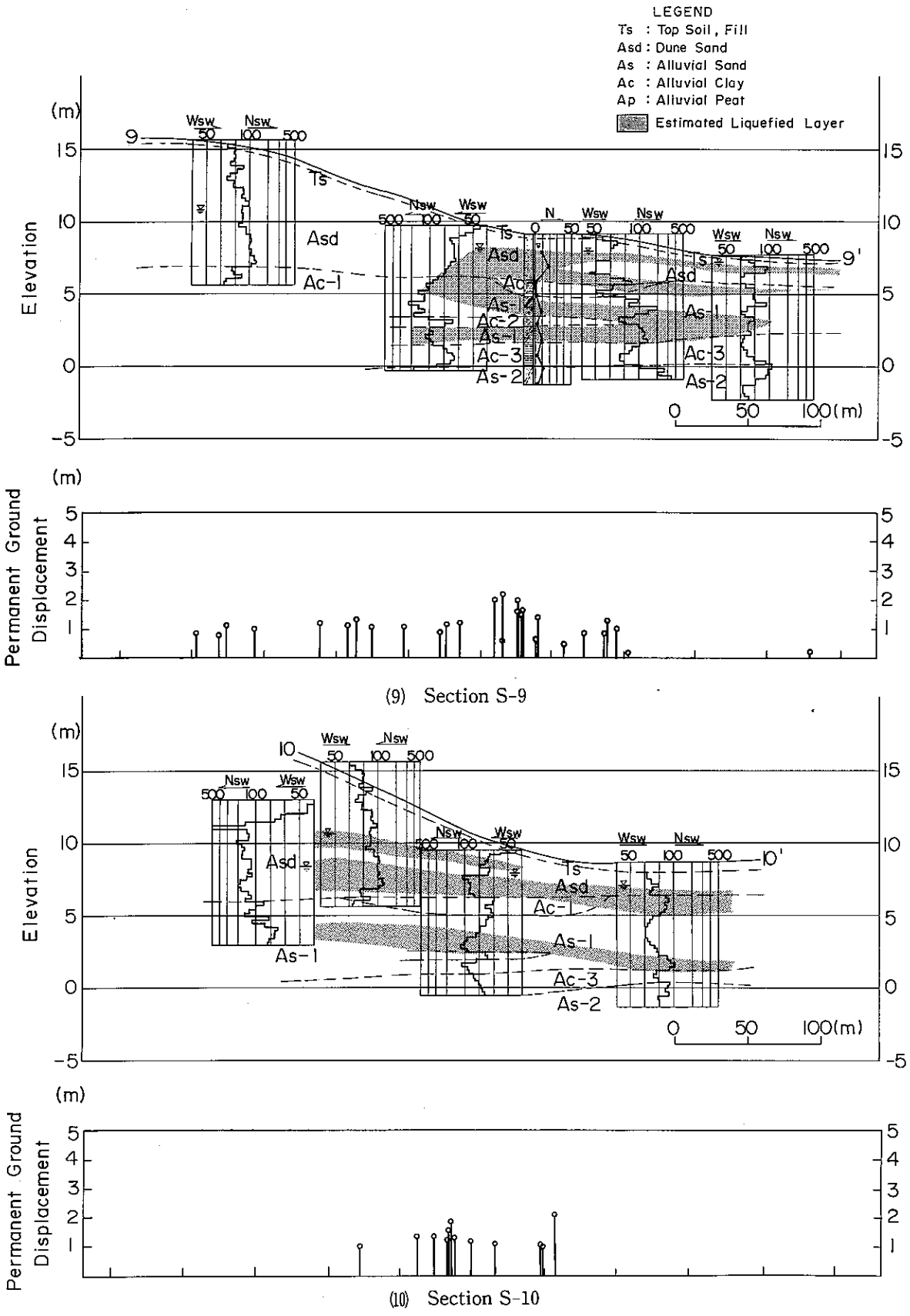
Fig. V-1 Soil layer profile in Noshiro City
