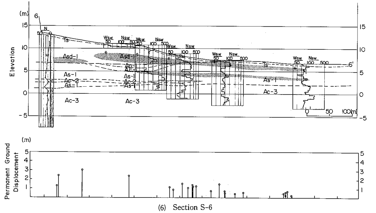
Fig. V-1 Soil layer profile in Noshiro City
